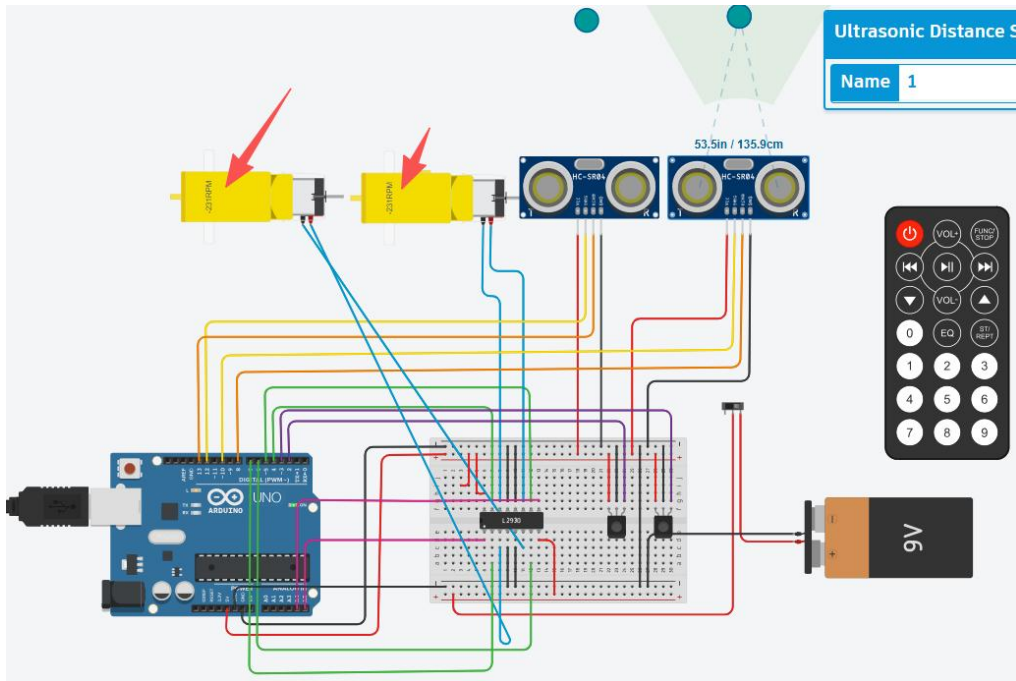
Figure 2 initial design draft in Tinkercad can function properly
