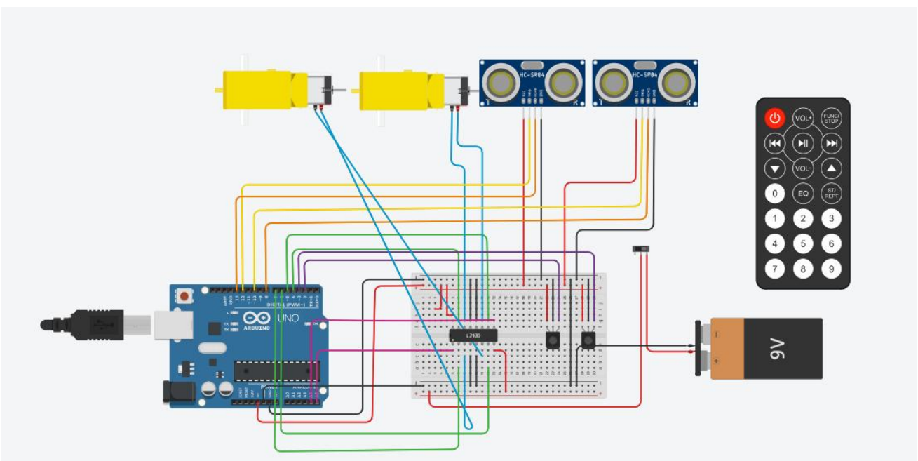
Figure 1 initial design draft in Tinkercad
